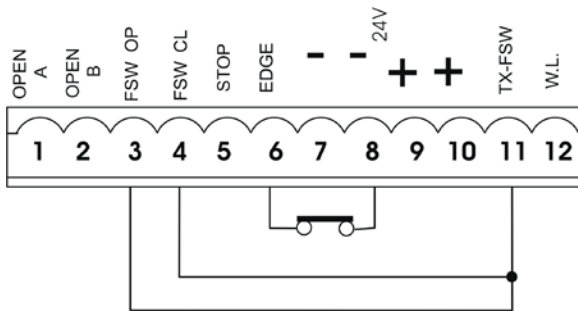
Connection of an "edge" safety device
